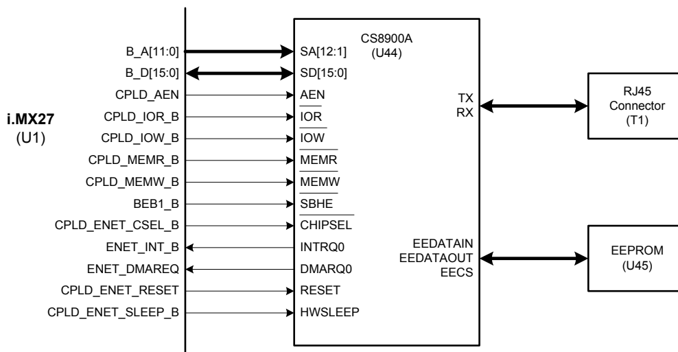
Figure 2-9. External Ethernet Interface
